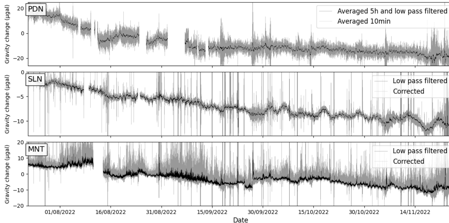
Gravity changes between July and November 2022
